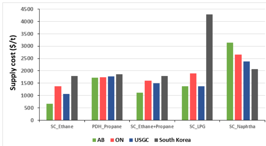
Figure E4: Indicative CTNC Supply Costs per Jurisdiction and Feed Type, Plant Gate (2018 Constant Dollars)
