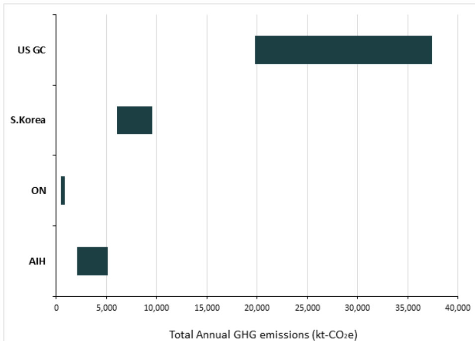
Figure E.6: Total Annual GHG Emissions from Petrochemical Hubs (2016 capacities basis)
